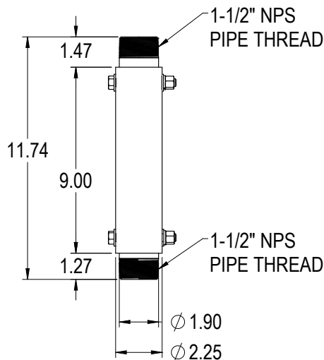
Speaker Mount
