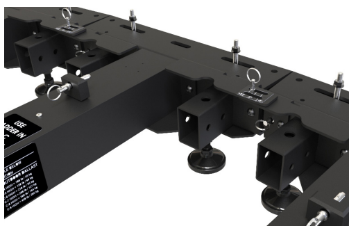
T-BASE Connection
