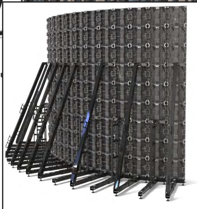
Single Column LED Framing
