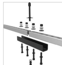
CG-P1377-JBX2 with threaded rod
