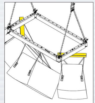
Cross Arms in yellow
